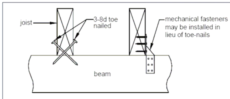
FIGURE 17: JOIST-TO-BEAM DETAIL
