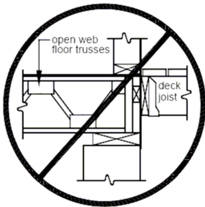
FIGURE 8: NO ATTACHMENT TO OPEN WEB TRUSSES
