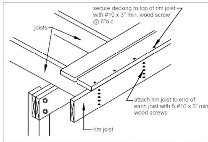
FIGURE 18: RIM JOIST CONNECTION DETAILS
