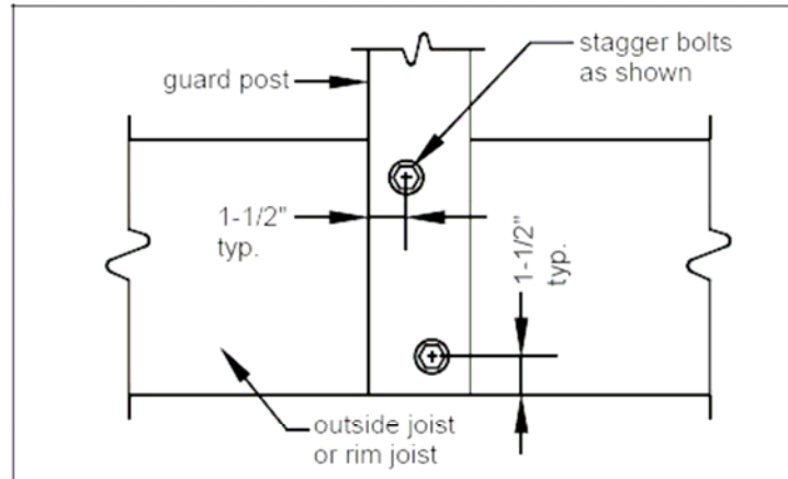
FIGURE 23: GUARD POST ATTACHMENT DETAIL
