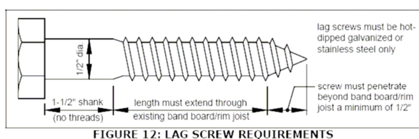
FIGURE 12: LAG SCREW REQUIREMENTS
