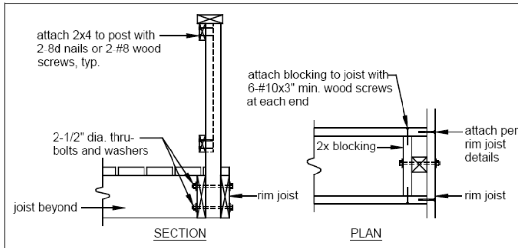
FIGURE 25: GUARD POST TO RIM JOIST DETAIL, OPTION 1
