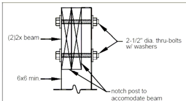
FIGURE 20: POST-TO-BEAM REQUIREMENTS
