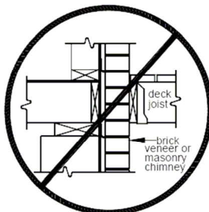
FIGURE 9: NO ATTACHMENT TO BRICK VENEER
