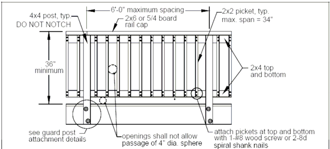
FIGURE 22: TYPICAL GUARD DETAIL
