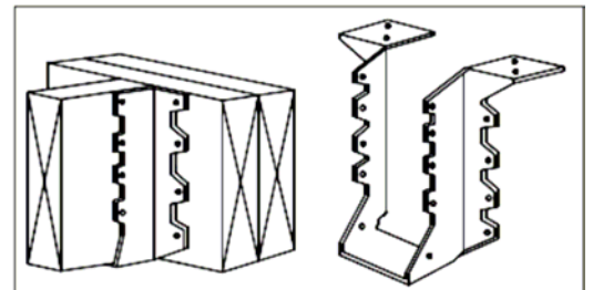
FIGURE 16: TYPICAL JOIST HANGERS
