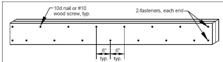
FIGURE 19: BUILT-UP BEAM DETAIL
