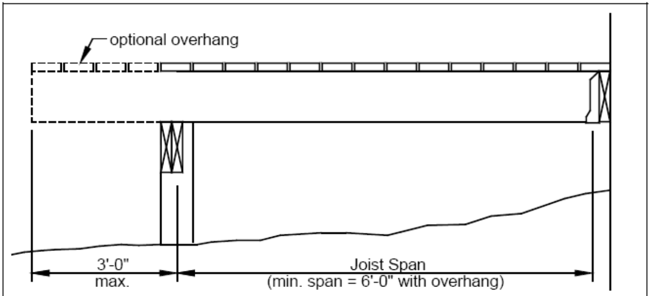
FIGURE 1: JOIST SPAN - DECK ATTACHED AT HOUSE
