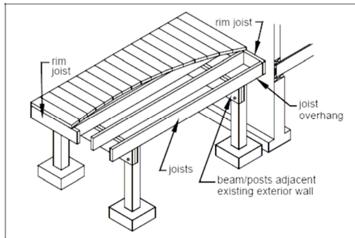
FIGURE 13: FREE-STANDING DECK
