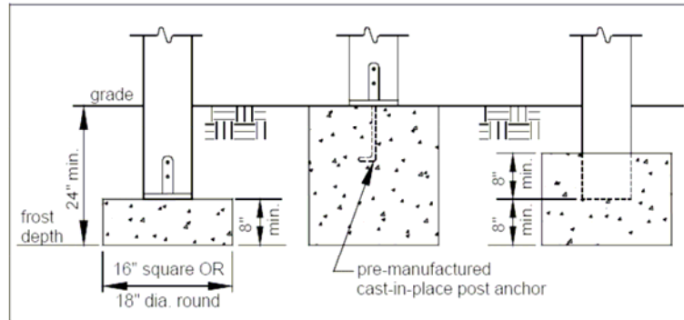
FIGURE 21: TYPICAL FOOTING DETAILS
