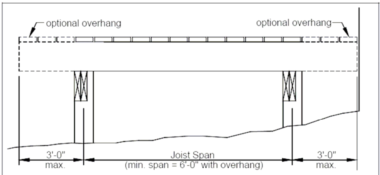
FIGURE 2: JOIST SPAN - FREE-STANDING DECK
