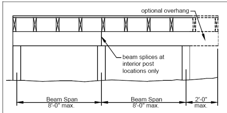
FIGURE 3: BEAM SPAN TYPES
