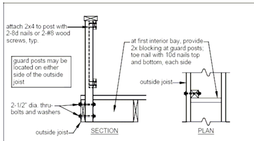
FIGURE 24: GUARD POST TO OUTSIDE JOIST DETAIL
